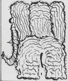
Loxodonta africana
