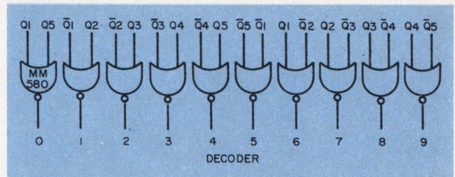
5. Each decoder converts the outputs of its Johnson counter to ten address lines, which are used to drive the multiplexer gates.
