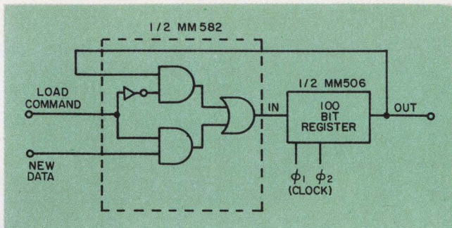
7. The 100-bit accumulator consists of a 100-bit shift register and gating elements. Information is routed into the register from the multiplexer and is then allowed to recirculate.
