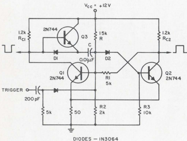
7. Faster retrigger time is obtained by adding a transistor and a diode, Q_3 and D_1 . The retrigger time of the one-shot of Fig. 6 ( 33 \mu\text{s} ) was reduced to only 5 \mu\text{s} . D_2 is added to protect the base-emitter junction of Q_2 .
