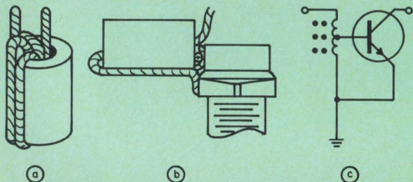
7. What could be simpler than this ferrite autotransformer (a)? To eliminate undesired parasitics, a special mount was designed to get the transformer right up close to the transistor (b). The schematic representation of this circuit is shown in (c).
