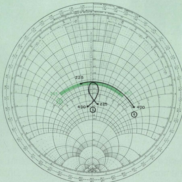
2. The large-signal input impedance of an ITT 3TE445 transistor is shown by curve (a) from 225 to 400 MHz. In (b), the effect of putting a capacitor in series with the base is shown. Curve (c) results when a shunt pole (Fig. 3) is added. All curves are normalized to a 1-ohm line.
