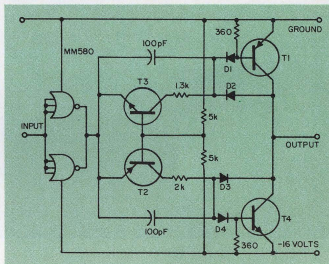
9. The output buffer is a push-pull complementary output stage which provides a high current drive capability and ensures 1-MHz operation of capacitive loads. An MOS input stage assures voltage compatibility with the output of the 100-bit shift register.
