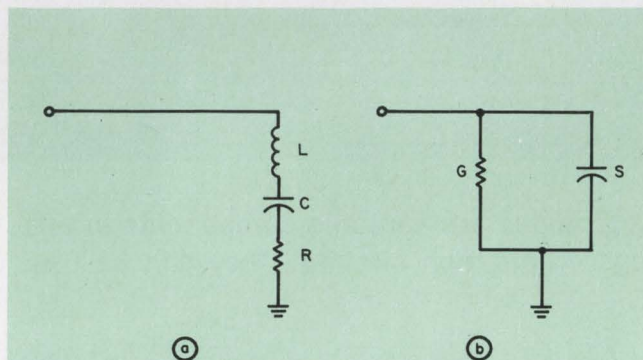
1. The large-signal equivalent circuits for the input (a) and output (b) of a typical rf power transistor contain both resistive and reactive elements. The circuit is a common emitter configuration with a series R-L-C equivalent for the base (input) and a parallel conductance-elastance equivalent for the collector (output).
