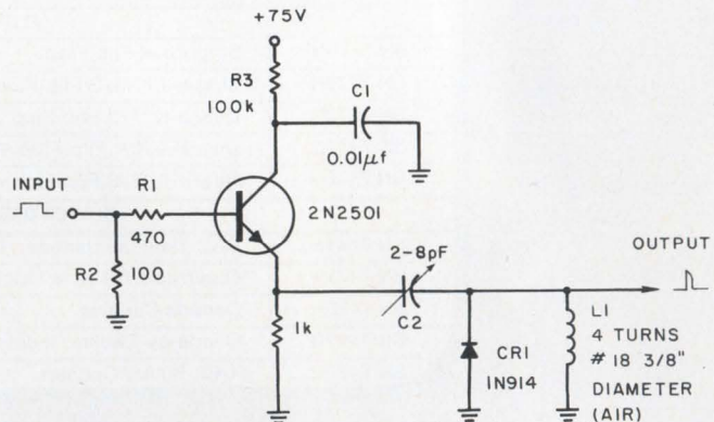
Very narrow output pulse is produced by this pulse differentiator each time a pulse is applied to the input.
