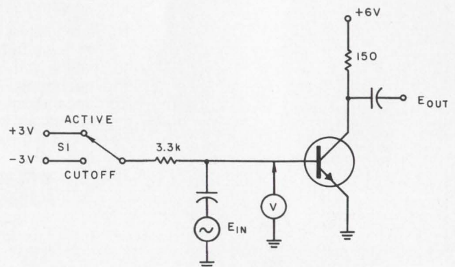
1. Basic switching action is performed by the transistor emitter-base diode.
