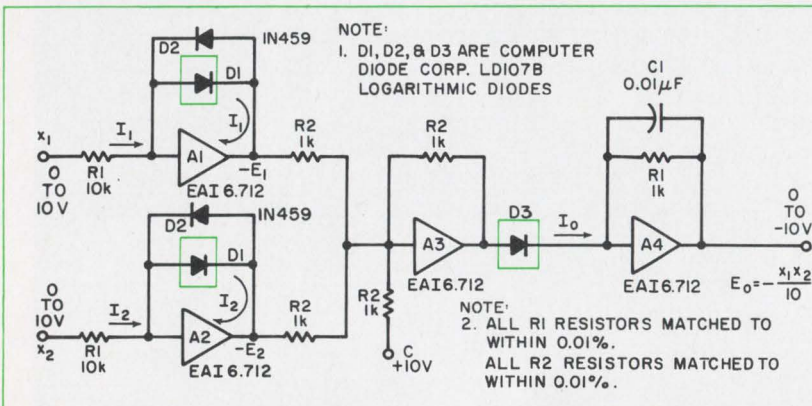
3. Complete multiplier circuit operates as follows: (1) it converts the input voltage into currents I_1 and I_2 , (2) it produces voltages E_1 and E_2 , which are the logs of currents I_1 and I_2 , (3) it sums E_1 and E_2 , (4) it takes the antilog of the sum of E_1 and E_2 to produce I_o , and (5) it converts I_o into the output voltage E_o .
