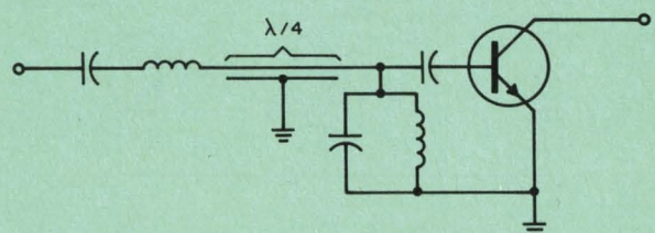
5. The series zero and quarter-wave line added to the circuit of Fig. 3, have transformed the input impedance to that of Fig. 4b.
