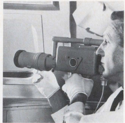
TV camera that sent back views of the moon and earth never seen before weighs 4.5 pounds, uses a 1-inch vidicon tube and pulls 6.7 watts. Built by RCA, it uses a 500-kHz bandwidth and provides 10 frames per second with a 320-line raster.
