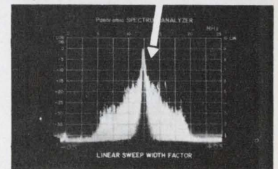
Expanded View of One Channel
