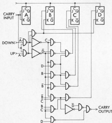
DTL implemented up-down counter
