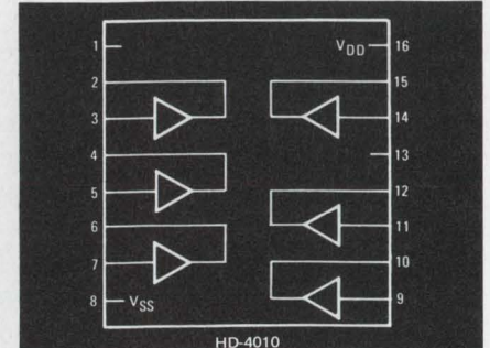
Pin for pin compatible with CD 4010A.
