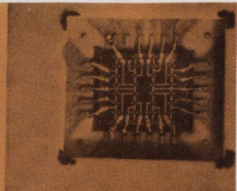
Fig. 4. Logic circuit based on Fairchild MOSFET is fabricated using all planar processes in a single silicon structure. Gate, drain, contacts of one MOS and the depletion-mode FET are etched in separate steps. Gate, drain, contacts and contacts are etched in separate steps.
