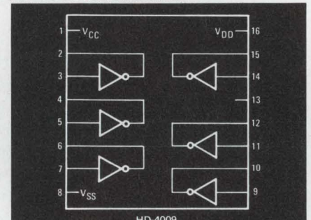
Pin for pin compatible with CD 4009A.
