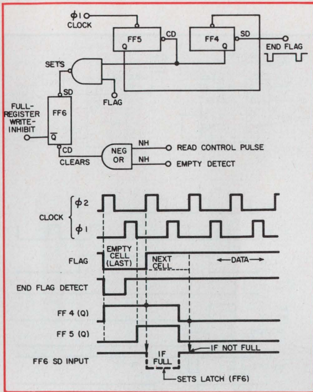
5. A completely full register of 100 characters would result in no flag transitions. Therefore at least one stage is always empty to insure an active flag signal.
