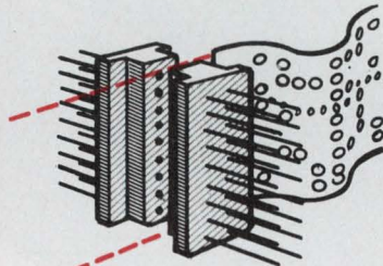
FPA 100 9-Element Source-Sensor Tape Reader Array
