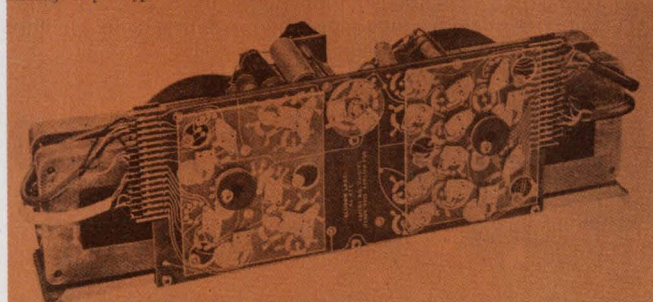
The Hartsack Etched Plate switch of Allison Laboratories, shown in an octave band filter assembly, was an early application of etched multilayer circuitry.
