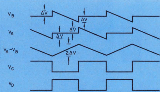
2. A voltage change \Delta V at nodes A and B does not change the frequency of square-wave outputs V c and V d .
