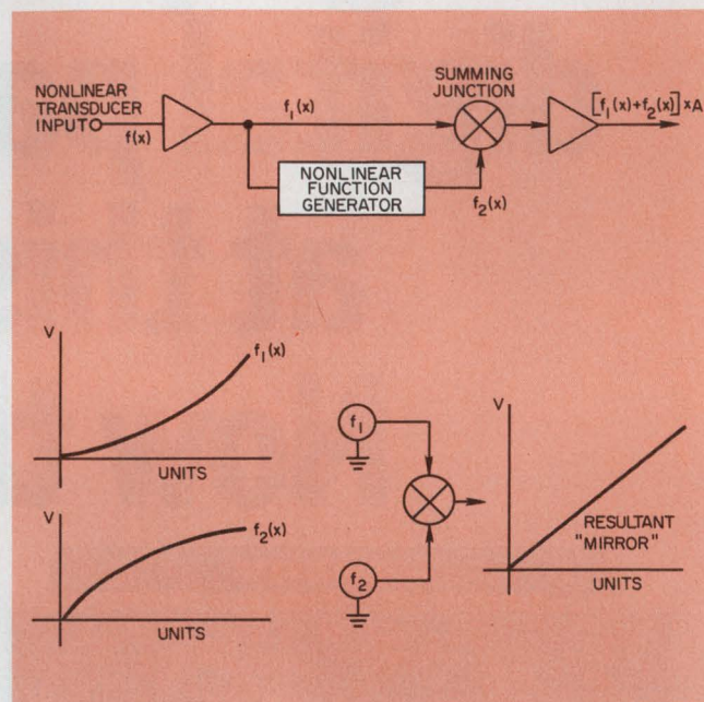
1. Analog functions are linearized with a simple circuit (a) that uses the original input functions to generate its mirror image, f_2(x) , shown in (b). After the original amplified function, f_1(x) , is added to f_2(x) , the desired linear output is obtained and it is called "mirror." Functions f(x) are voltages generated in response to some physical variable "x," which might be temperature, pressure, velocity, etc.
