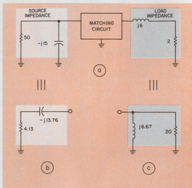
1. The first step in matching impedances is to convert the source and load impedances (a) into the most convenient form for doing the subsequent calculations. Parallel configurations (b) can be converted to series, and vice versa (c), depending upon use of an L, T or Pi.
