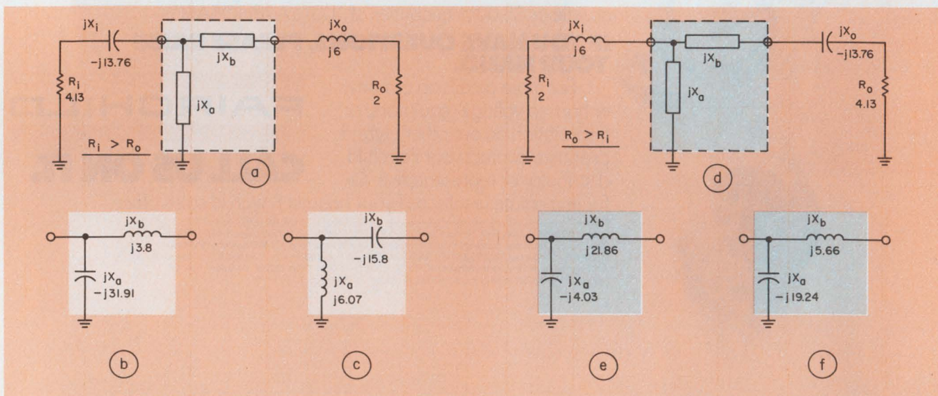
2. An L-section matching circuit (a) can have two solutions—a low (b) and high-pass form (c)—when R_i > R_o .
