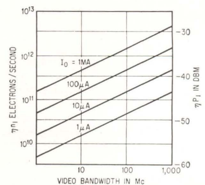
MINIMUM DETECTABLE NUMBER of electrons/sec and minimum detectable power at 7,000 A, both multiplied by \eta , are shown for an amplitude-modulated microwave phototube—Fig. 5
