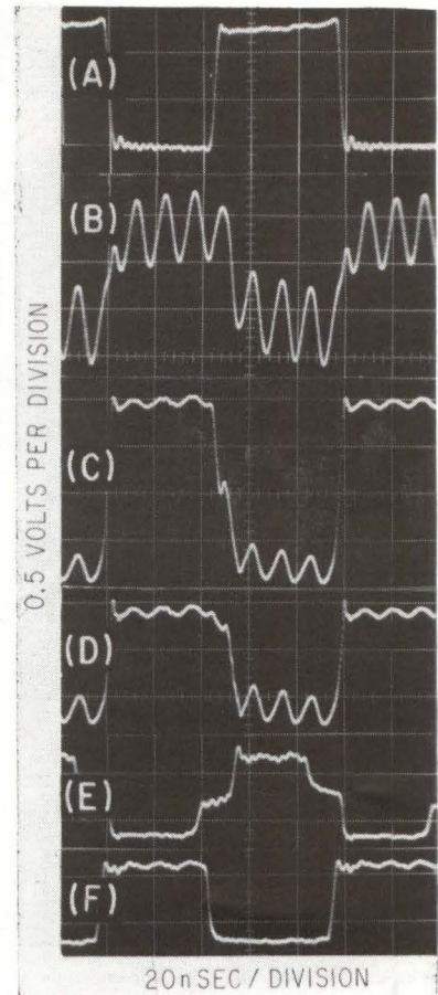
WAVEFORMS ARE FOR 80-Mc to 10-Mc division. Letters (A) to (F) refer to measurement points denoted by callouts on Fig. 1A—Fig. 3
