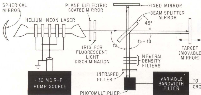
MULTIPLIER PHOTOTUBE noise determines system signal-to-noise level
