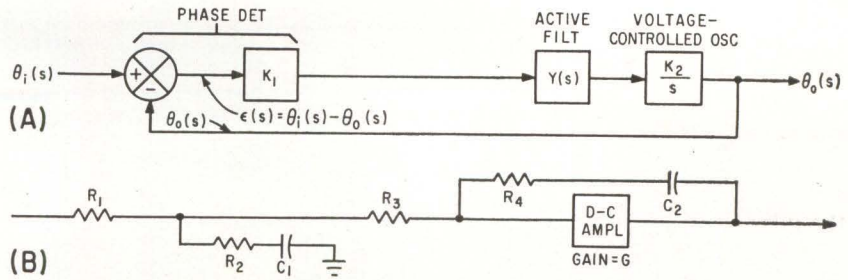
MATHEMATICAL MODEL (A) of phase loop. Circuit of active filter is shown in (B)—Fig. 4
