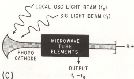
USING MICROWAVE PHOTOTUBE as a detector of a-m light (A). First experimental X-band phototube (B). Using a microwave phototube as a mixer (C). Tube shown in (D) is similar to (B) tube—Fig. 1
