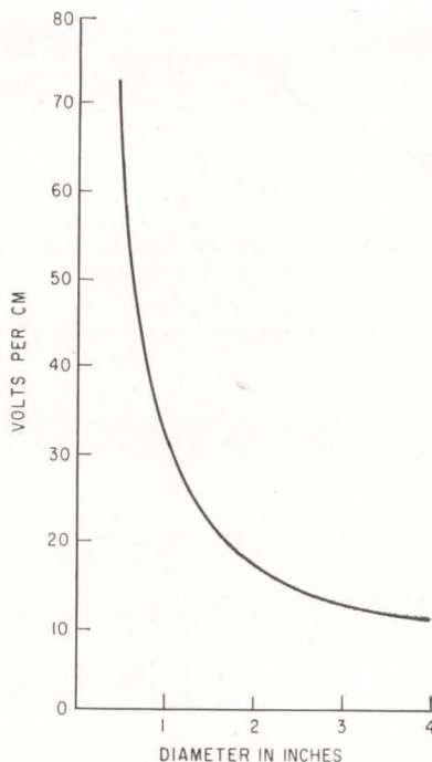
SENSITIVITY of helium-neon ion orb is shown as a function of orb diameter—Fig. 2
