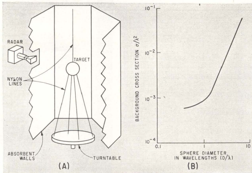
TYPICAL C-W TEST range (A) is a radar darkroom. Range sensitivity versus sphere is shown in (B)—Fig. 2
