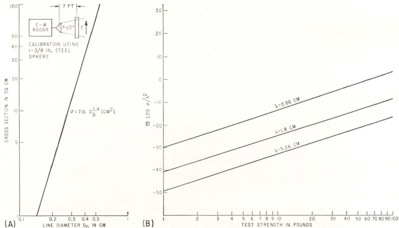
DETERMINATION OF NYLON line cross section at X-band (9.2 Gc) (A) and estimated cross section of nylon line as a function of test strength and radar frequency—Fig. 4
