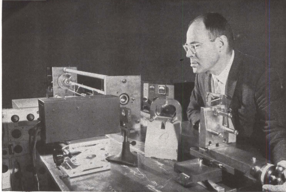
EXPERIMENTAL doppler laser uses continuous-wave gas laser recently developed by Sperry
