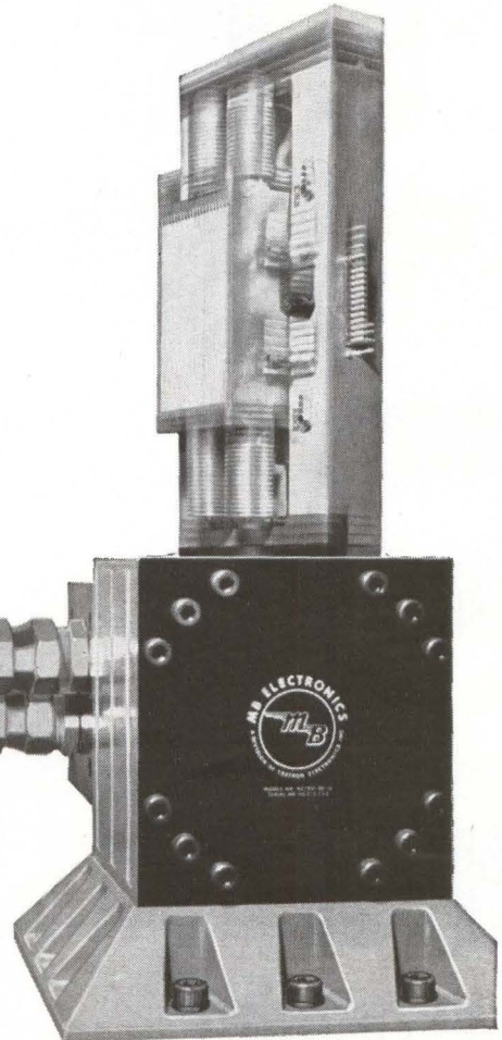
View of typical MB hydraulic actuator with a force rating of 100,000 lbs. Measures only 18" x 18" x 13".
