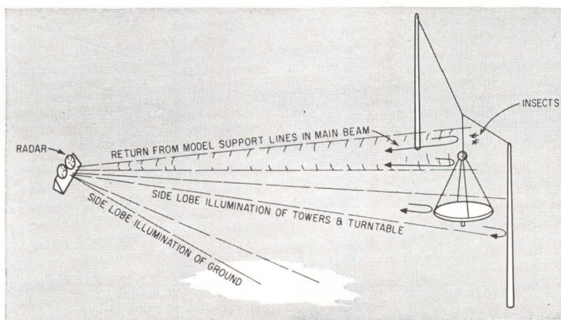
PULSE MEASUREMENT cross section range showing sources of extraneous returns—Fig. 3
