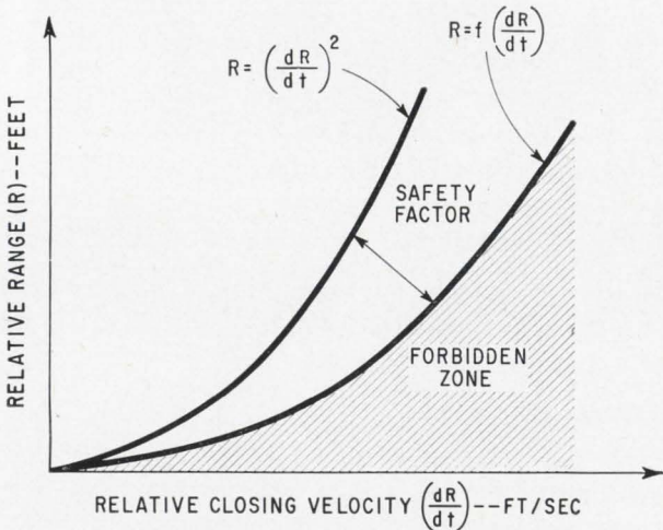
Flight profile is relation between range and range rate of approach of the two vehicles. Optimum profile would result from a deceleration that results in zero range at the instant the range rate of approach is also zero. Engine thrust determine the flight profile. Forbidden zone indicates a profile that would cause spacecraft to pass the target without docking.
