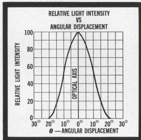
Figure 6. Narrow beam width from TIXL01 minimizes optical cross-talk and light shielding.
