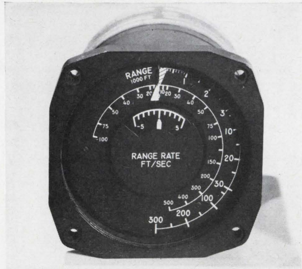
Range and range-rate indicator observed by astronaut who maintains a safe deceleration rate by keeping the range-rate pointer below the range pointer. When R and dR/dt pointers are aligned, the spacecraft is on an R = (dR/dt)^2 deceleration profile. Vernier scale provides finer range rate resolution required when the vehicles dock.
