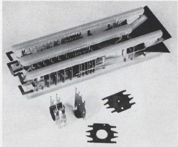
Lugs at corners of disks are inserted simultaneously into six glass rods to form the double-gun assembly.
