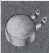
M2 Narrow Diff. Thermal Switch 2^\circ to 5^\circ\text{F} differential in 0^\circ to 250^\circ\text{F} range.
