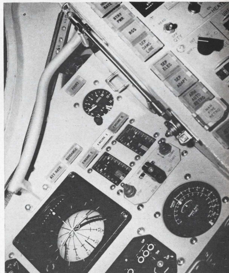
Variables monitored (left) by the malfunction detection system are related to the actual pilot displays (right) in the Gemini capsule. "Att. Rate" light goes on when Gemini turns at an attitude rate beyond safe value. "Guidance" light is illuminated switchover to secondary guidance and flight controls. Engine lights are energized when thrust is lost, and meters indicate gas pressures in propellant tanks.
