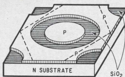
Complete mask-epitaxy transistor is at left. At right is the first junction made in the same transistor. Transistors are separated along dotted lines.
