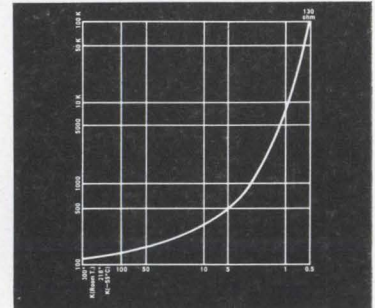
Log graph shows resistance-temperature characteristic of Speer 130-ohm carbon resistor between 300^{\circ}\text{K} and .1^{\circ}\text{K} .
