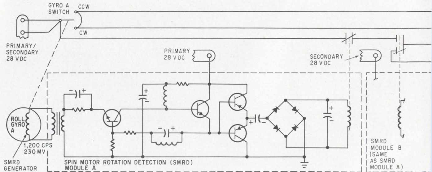
Gyroscope measures turning rate of launch vehicle. When turning rate exceeds safe value, contacts close and a 28-volt d-c signal i
