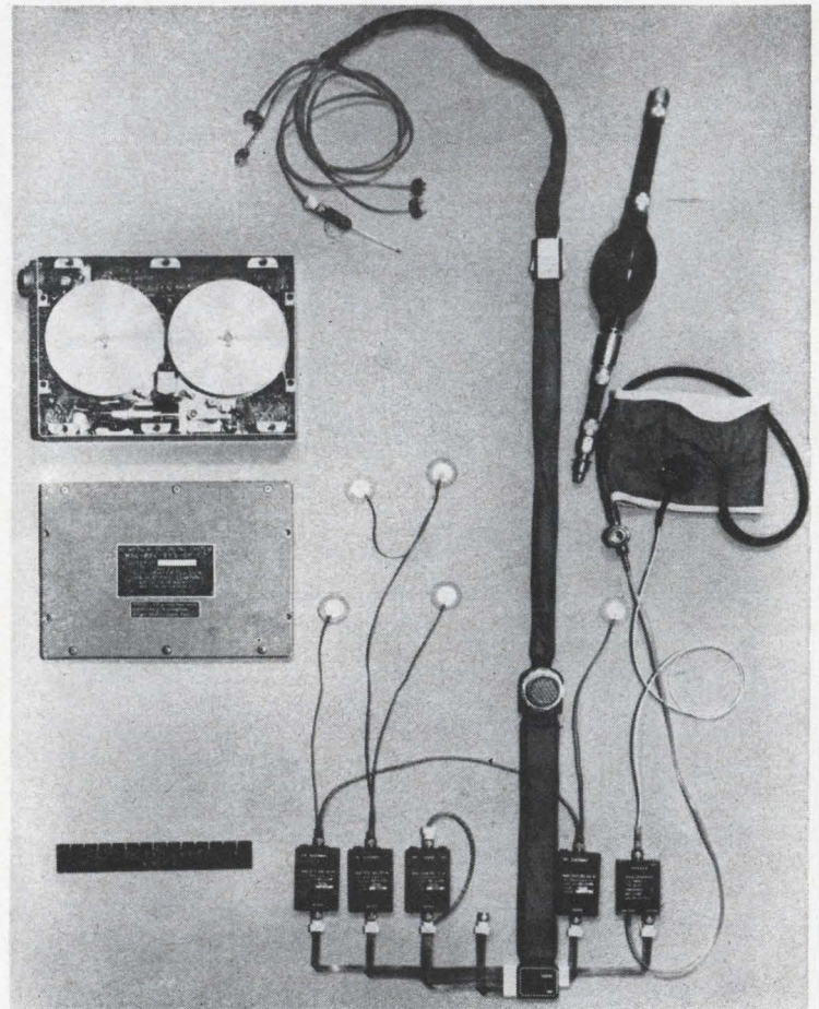
All sensors and signal conditioners are connected to a common trunk cable. The large connector in the center of the trunk provides a breakout point from the space suit. The miniature tape recorder, capable of recording for 100 hours, is in the top left corner.
