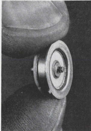
Figure 2. New TI-designed coaxial package for TIXS12-13 high-frequency transistors.
