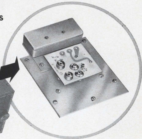
TRANSISTOR TEST JIG TYPE 13510A
