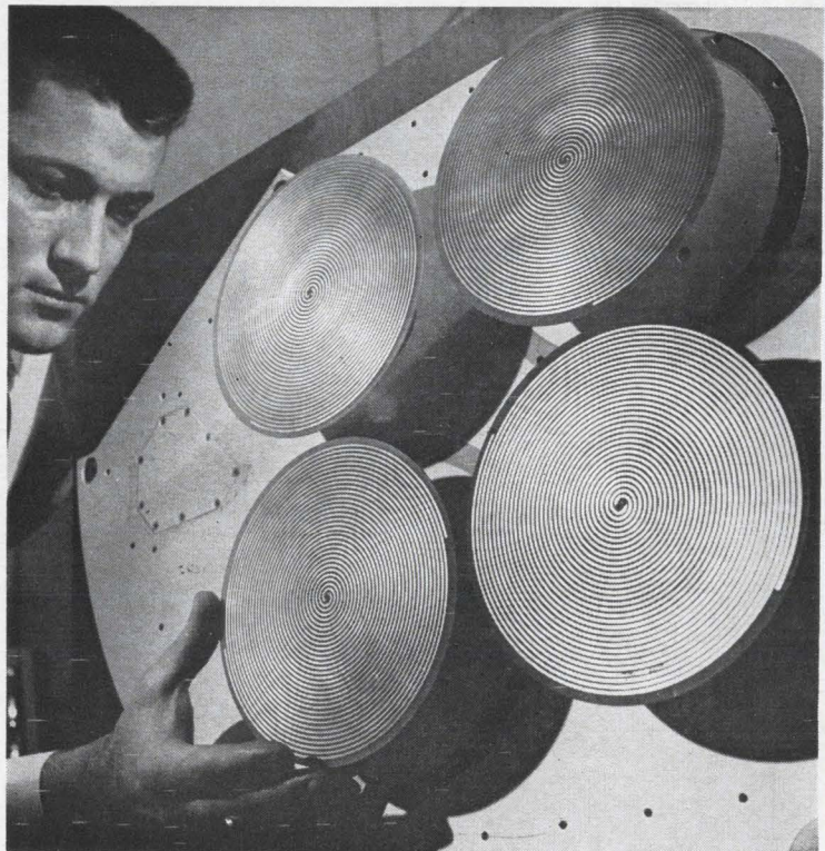
Antenna system consists of circularly polarized antennas in the form of Archimedian spirals, printed directly on epoxy boards. One transmitting antenna and three receiving antennas—azimuth and elevation measurements share a common antenna—shown by Westinghouse engineer, O. Lamar Bishop, are in the front of Gemini. Transmitter antenna and common receiver antenna are fixed, while the azimuth and elevation receiver antennas can be rotated.
