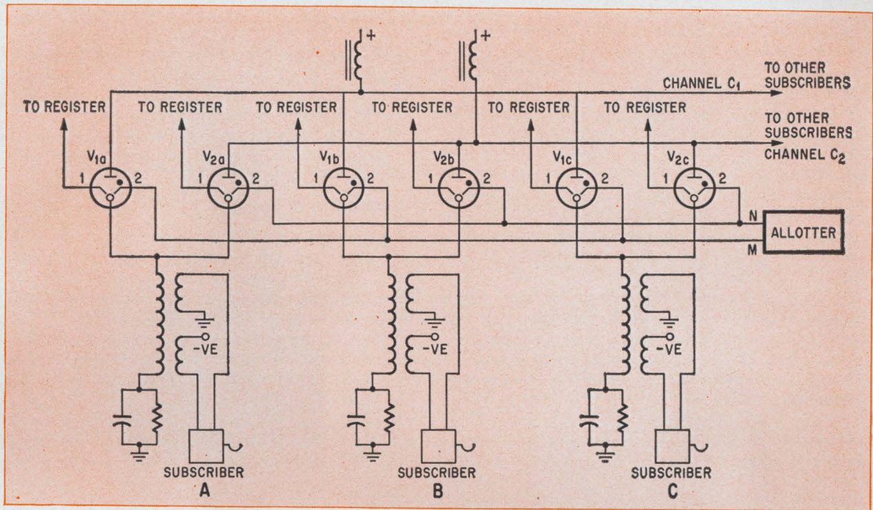
▲ Basic circuit of automatic telephone exchange. Each phone is connected to common channels through a trigger tube.
