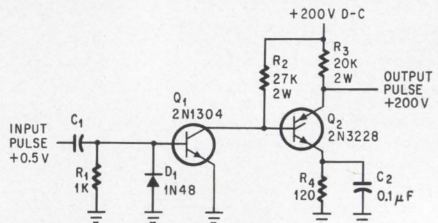
Low positive input pulse causes Q_1 to conduct and switches gate of scr 2 volts negative with respect to cathode.
