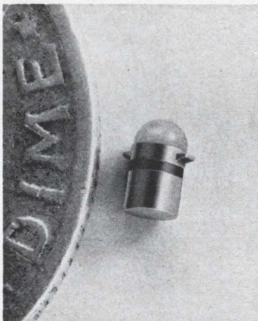
Figure 5. TIXL01 solid-state light source. Unit mounts directly in 1/16 in. printed circuit board.
