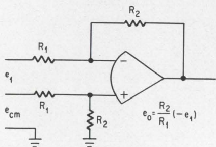
Differential or difference amplifier
