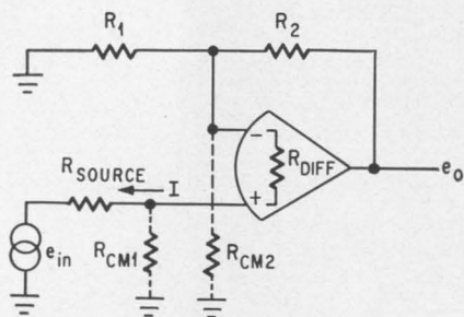
Buffer connection for differential operational amplifier
