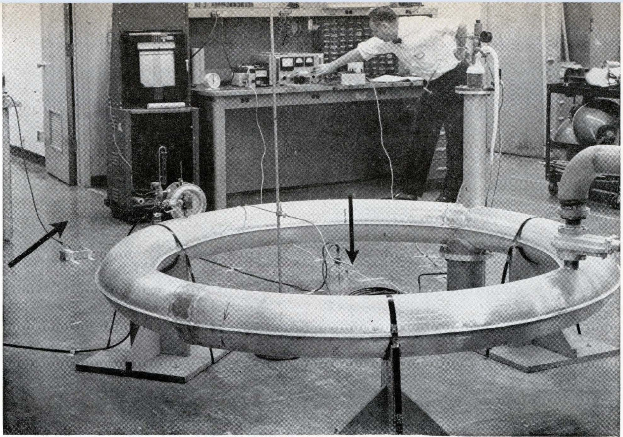
Six-foot diameter superconducting coil used to study radiation shielding. The black arrows are stamped steel pieces that are being supported by the magnetic field.
