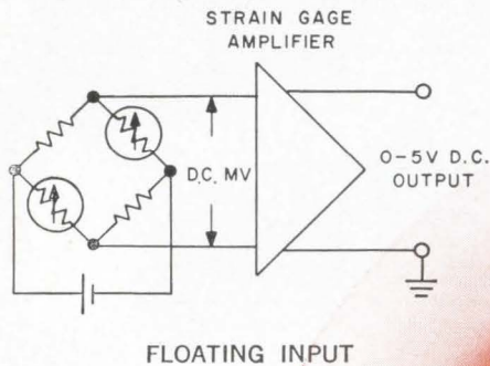
STRAIN GAGE AMPLIFIER FLOATING INPUT
