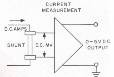
CURRENT MEASUREMENT HIGH-SIDE MONITORING
