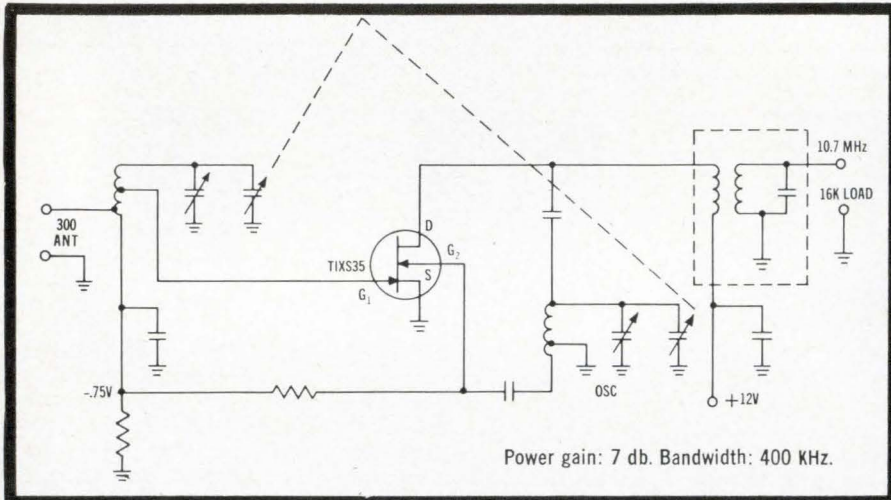
1. Unique autodyne mixer employs TIXS35 FET which functions as both mixer and local oscillator.
