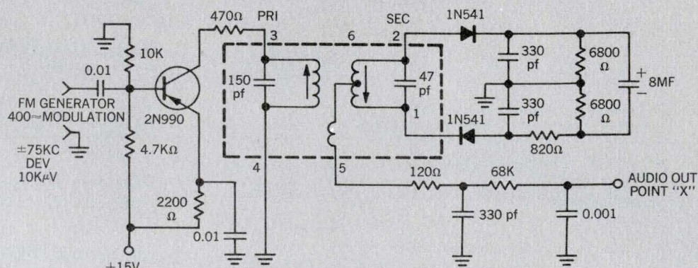
FM RATIO DETECTOR
