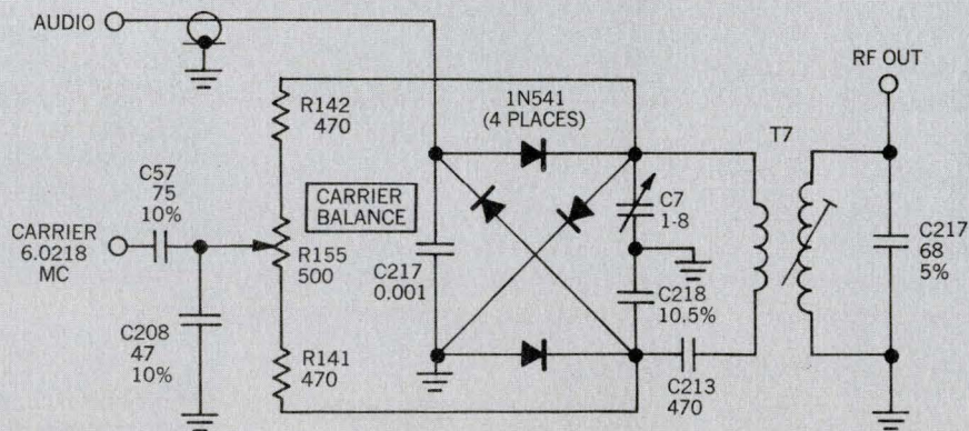
BALANCED MODULATOR CIRCUIT
