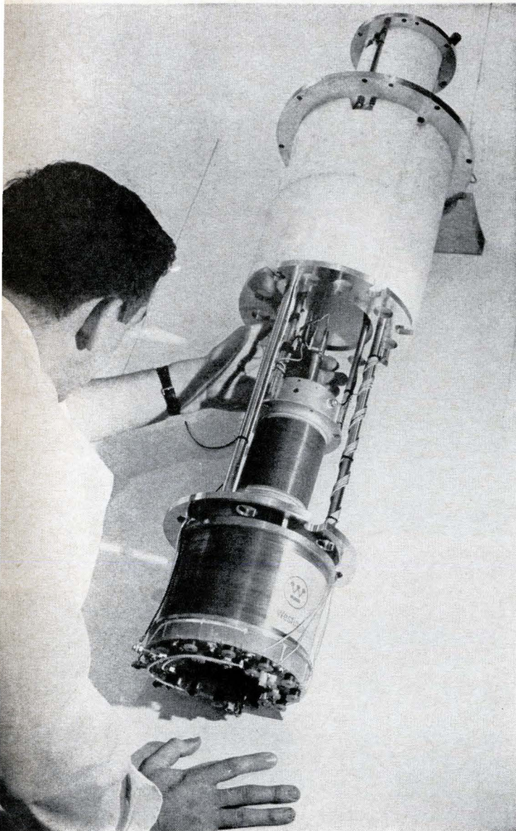
A 100-kilogauss superconducting magnet. Three concentric magnets were used to produce the field; the smallest one is shown next to the researcher's left hand.
