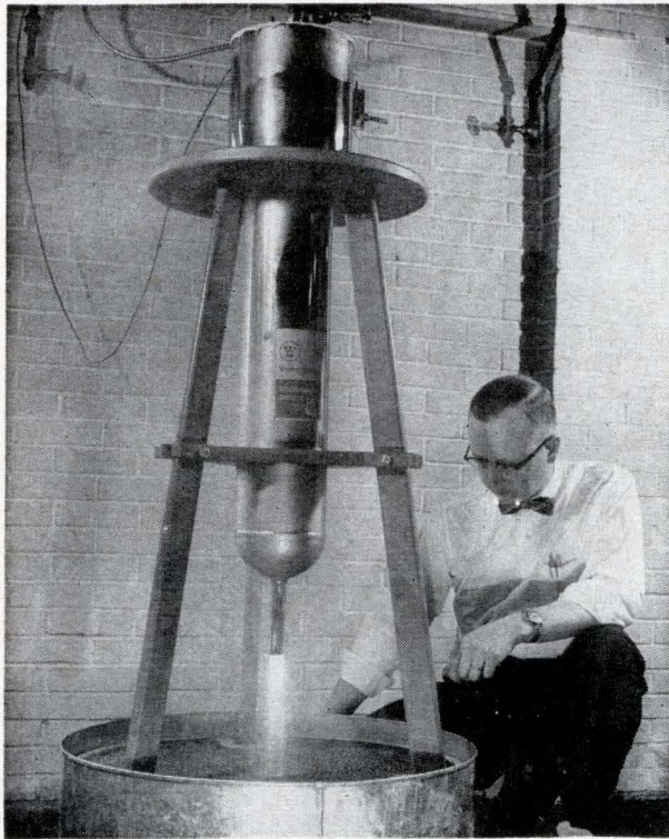
Magneto hydrodynamic (MHD) generator uses a 1-inch air-core superconducting coil for the field coil. The coil and its support are being lowered into the Dewar vessel.
