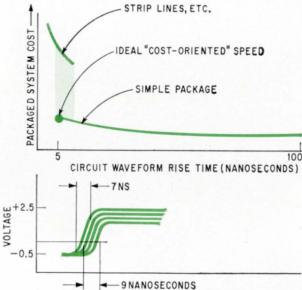
Strip transmission-line interconnections , a costly packaging technique, are required for logic speeds faster than 5 nanoseconds. Two-sided boards can be used at slower speeds (top graph). Emitter-follower circuitry allows stage delays of about 3 nanoseconds (lower graph) in the simpler package form.
