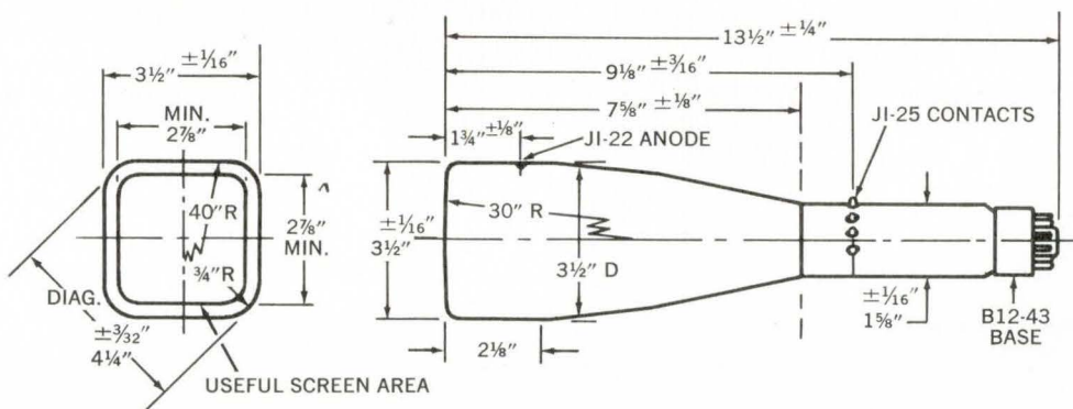
SC-3511, SC-3377, and SC-3551 Outlines
