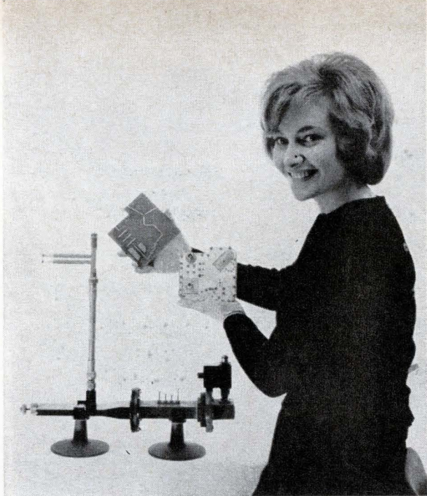
Comparison of equivalent microwave and strip transmission line circuits shows the reduction in size offered by the latter technique. Girl holds both the basic strip transmission line circuit board and the complete package for a varactor tripler.
