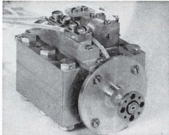
Traveling-wave maser has a superconducting field coil that is housed in the metal section attached to the left side of the maser.
