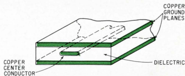
In a typical strip transmission line, a center conductor guides electrical energy between two conducting ground planes. Here the thickness of the center and ground planes has been greatly exaggerated.
