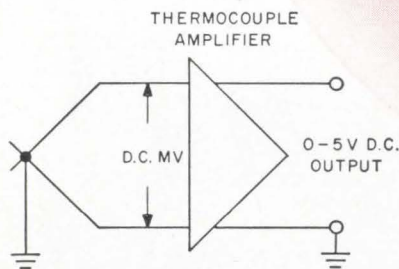
THERMOCOUPLE AMPLIFIER ISOLATION OF GROUNDS
