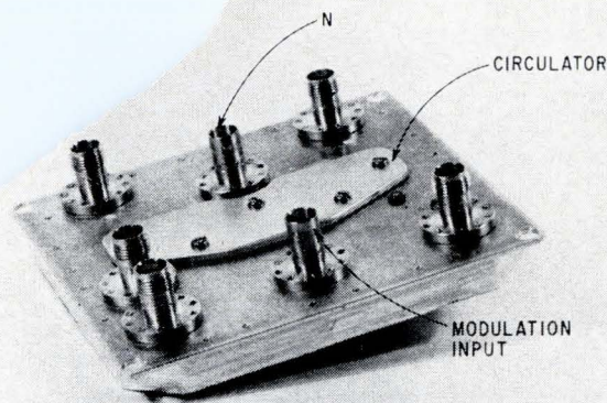
Five-port diode switch allows the output to be modulated by a single source. The five connectors, which are not marked, are the output ports. An input connector and the diode bias lines on the bottom of the switch are not visible. The port marked N is not a part of the switch.
