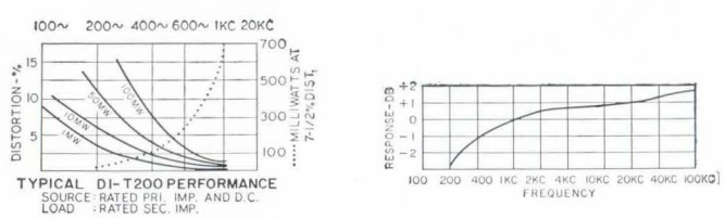
TYPICAL DI-T200 PERFORMANCE SOURCE: RATED PRI. IMP. AND D.C. LOAD - RATED SEC. IMP.
