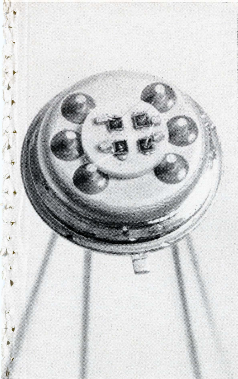
Multichip transistor multiplier contains four silicon planar epitaxial, pnp transistors in a TO-5 case.
