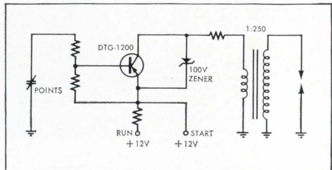
Automobile ignition circuit with the DTG-1200.
