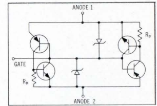
Silicon Bilateral Switch Equivalent Circuit
