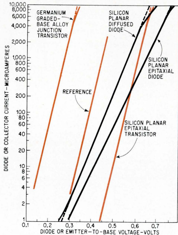
Diodes and transistors exhibit exponential characteristics represented by linear section of this semilog plot. Transistor curves, in color, have a slope equal to qV/kT . Reference line parallel to transistor curves is computed from equation 1 for an ideal junction at 298°K.
