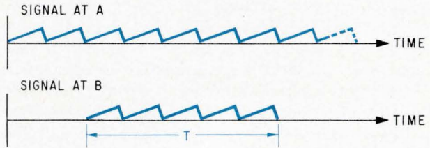
In an integrating dvm the time interval, rather than the frequency, is fixed. The unknown input voltage is converted to a proportional frequency, which is counted for a fixed period.
