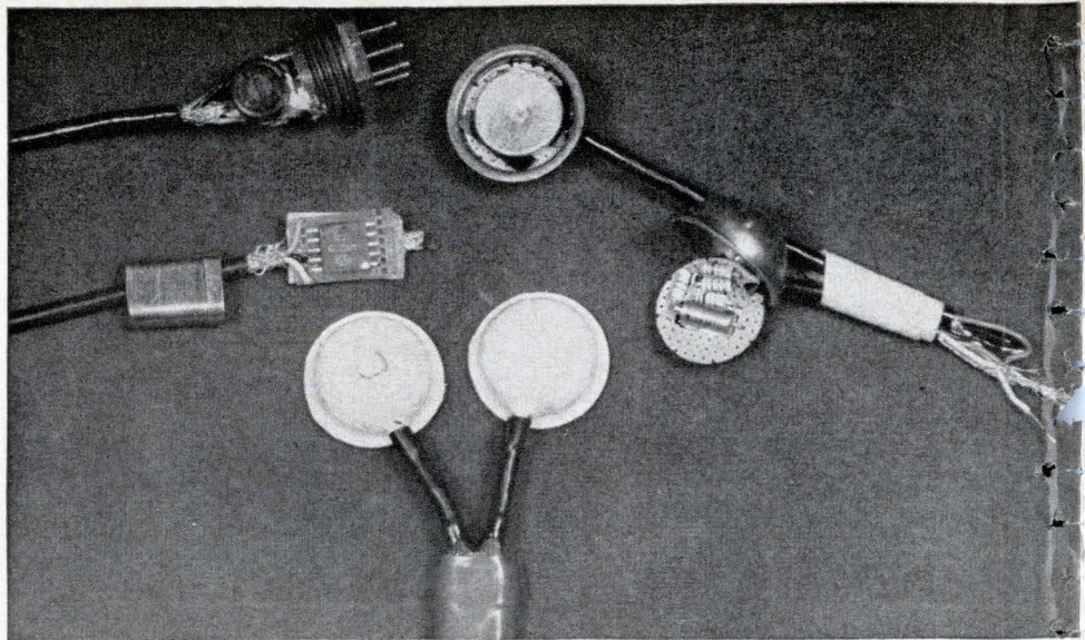
Differential electrodes, top and bottom views. Blocking capacitors behind each electrode prevent any d-c component from appearing at the signal processor.
