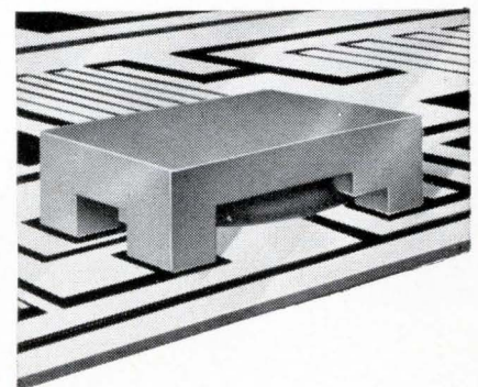
LID mounted on circuit
