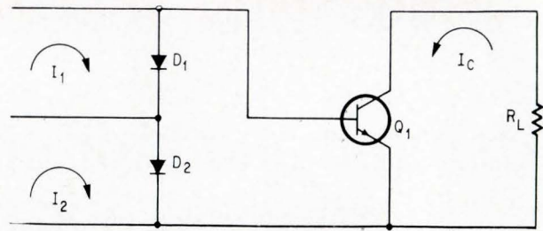
In simple multiplier, the voltage across D_1 and D_2 is proportional to \log I_1 I_2 . Collector current I_C is proportional to I_1 I_2 .
