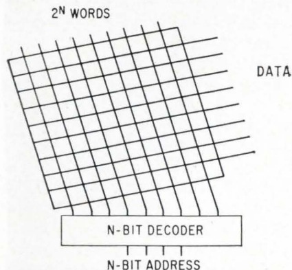
Two-dimensional organization is fast but quite expensive for large memories.
