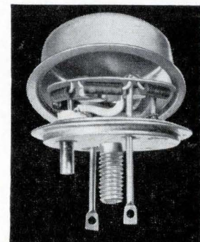
This is the super/reg ® synthesized zener diode.
