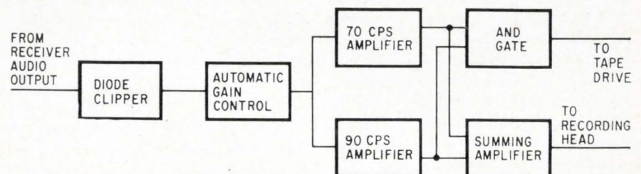
Dutch tape recorder runs for five seconds after frequencies from both selective amplifiers appear simultaneously at AND gate to trigger monovibrator circuit that powers tape drive motor. Prototype version shown above has two channels; production model will have three.
