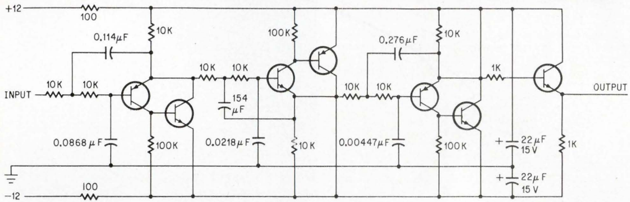
Active low-pass filter with constant phase shift
