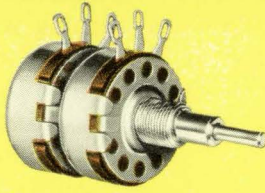
Type JJC dual unit with concentric shaft
