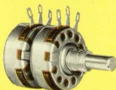
Type JJV dual unit with vernier adjustment
