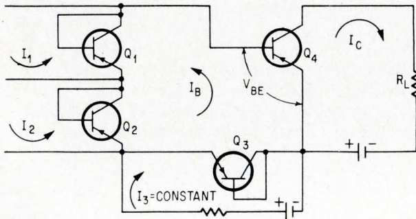
Practical multiplier adds circuit consisting of Q_4 and its current supply to permit increased input levels and to provide thermal compensation.
