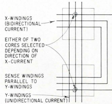
Bidirectional current is part of address decoding in 2 1 / 2 -dimensional scheme.
