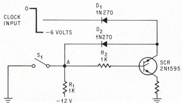
Adding latching feature to diode gate allows output to follow clock input when S_1 is closed. When S_1 is opened, output will be fixed at existing clock level.
