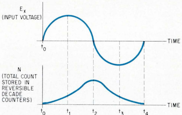
Integrating dvm has high immunity to noise since a-c signals are averaged out by reversible decade counters in the instrument. The number of counts builds up during one-half of the sine wave. But during the second half of the cycle, the counts are subtracted. The net count is zero.
