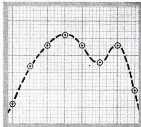
Point-by-point plotting with a signal generator
