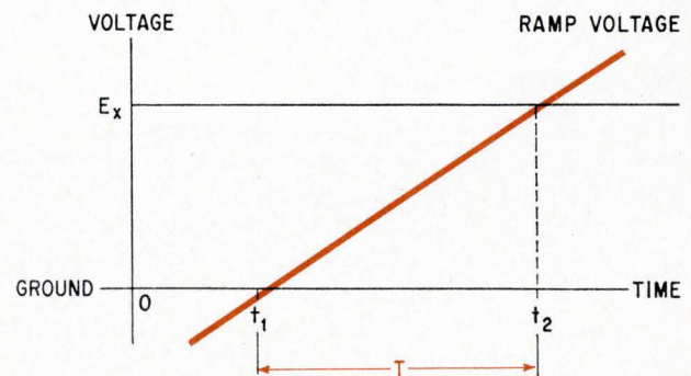
D-c voltage is measured with ramp technique by counting the number of cycles allowed through the gate during the time ( T = t_2 - t_1 ) the ramp voltage requires to increase from ground to the unknown voltage E_x .
