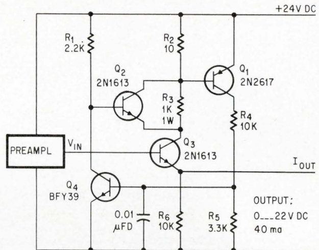
Electronic fuse in d-c amplifier cuts in high series resistance R_3 when there is an overload or short circuit and bypasses R_3 instantly when they are removed. All resistors 0.5 w unless otherwise specified.
