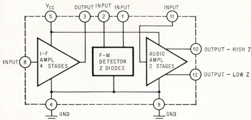
Hybrid integrated circuit television sound module.
