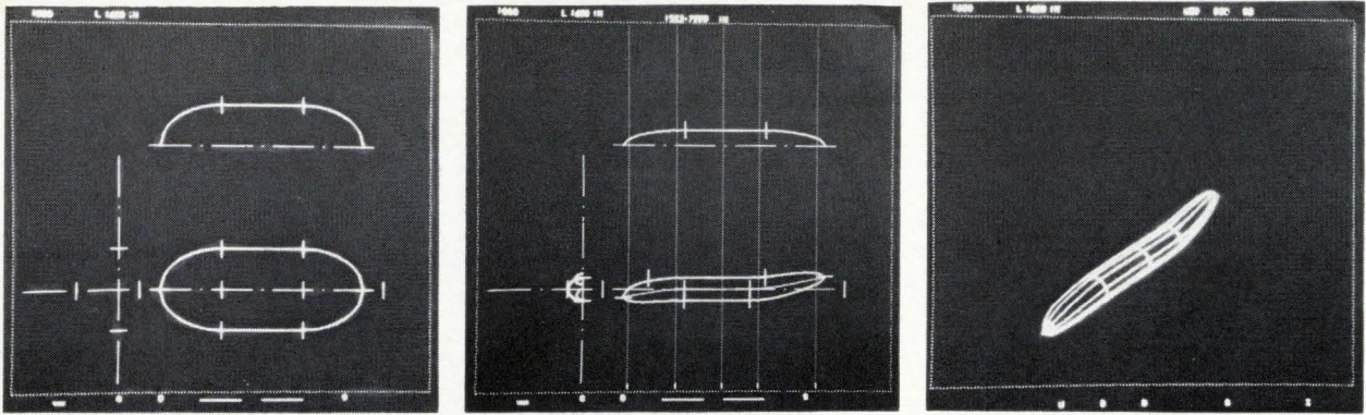
Cathode-ray tube display at Lockheed-Georgia shows design progression starting with basic surface (left) that is then shaped (center) and finally displayed in perspective.
