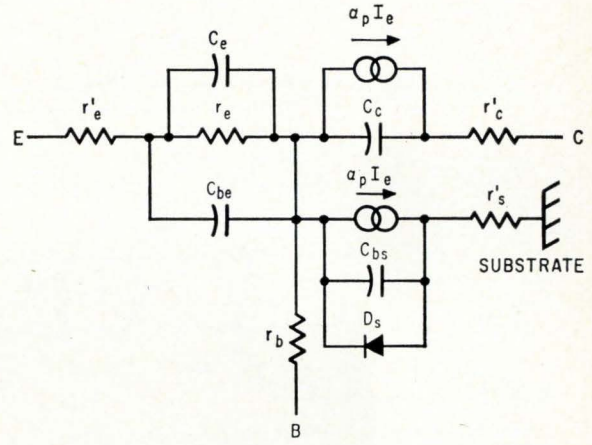
pnp EQUIVALENT CIRCUIT
