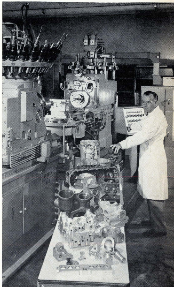
Machining centers made possible by numerical control perform a variety of tasks. One of the tool heads, upper left, on Hughes Aircraft's MT-3 unit holds 30 tools. It can change from one tool to another in less than 3 seconds.
