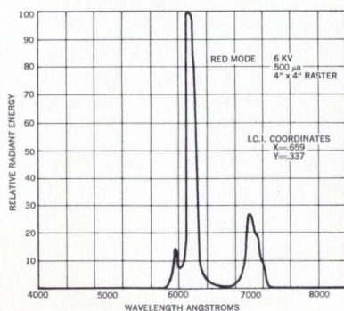
SPECTRAL ENERGY DISTRIBUTION (PHOSPHOR TYPE "PSO")
