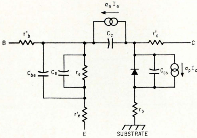
nnp EQUIVALENT CIRCUIT
