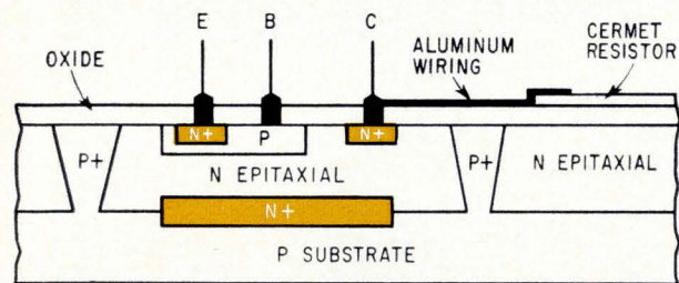
CROSS-SECTION
