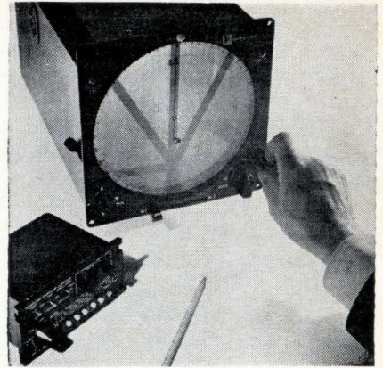
On the map. Computer-controlled display in Concorde navigation system shows aircraft's position on a chart.
