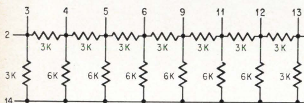
Voltage reference signals are formed by the ladder adder. An 8-bit element, it is fabricated on a 0.210 x 0.230-inch substrate using thin-film nichrome resistors on a glazed alumina substrate.
