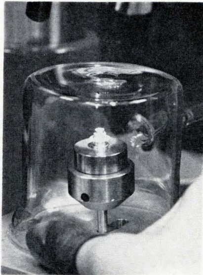
Light welder. A stainless steel jig aligns components for a miniature klystron as a laser beam bonds the parts. The glass bell jar holds argon, which prevents oxidation of the components during the welding operation.
