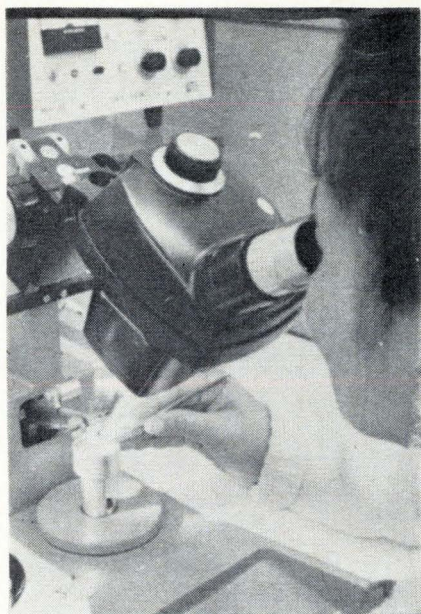
Eagle eye. Worker bonds flatpack assembly in Hewlett-Packard's integrated-circuit facility.
