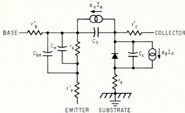
EQUIVALENT CIRCUIT
