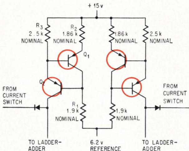
Dual-gated current source drives the ladder adder. Note that the npn-pnp piggyback configuration of the master level shift circuit is used.
