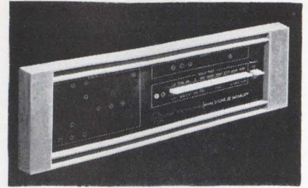
Compact. Core memory fits in standard rack space. The front panel includes self-test switches and indicators.
