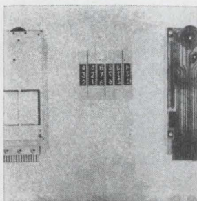
Commutator count modules are single digit pulse advance units for printing or reading. They also signal the position to which stepped by a rotated brush location against a commutator board. The printing or indicating wheel can be instructed to stop at any desired position when continually pulsed. Code is either 1 out of 10 or 12. Practical Automation Inc., Shelton, Conn. [426]
