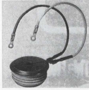
Full capacity thyristor type 282, designed to replace parallel scr's, permits upgrading of equipment with a minimum of external protection. When the device is water cooled, its rms current is 850 amps. Turn-on time is typically 5 μsec. I 2 T is 200,000 amps squared seconds, and forward and reverse voltages range up to 1,500 v. Westinghouse Semiconductor, Youngwood, Pa. [437]
