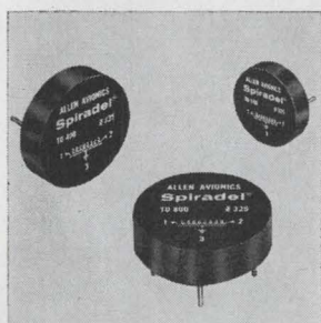
Distributed constant, fixed delay lines called Spiradel are compact and encapsulated for maximum environmental protection. Time delay to rise time ratios of over 20 to 1 can be achieved, with excellent temperature stability and pulse fidelity. Units cover a delay range of 100 to 1,000 nsec. Standard impedance is 325 ohms \pm 10\% . Allen Avionics Inc., E. 2nd St., Mineola, N.Y. [342]
