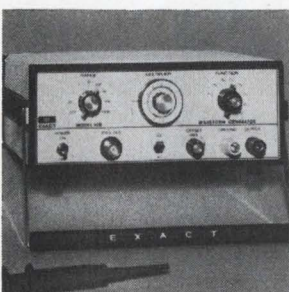
Waveform generator model 100 features miniature size (7.38 x 2.85 x 8.50 in.) and handle/tilt-stand. Frequency range is continuously variable from 0.001 hz to 3 Mhz, with square and triangle outputs to 5 Mhz. Output signal amplitude is \pm 5 v peak for positive and negative square-waves, 20 v p-p for all others, into a 600-ohm load. Exact Electronics, Hillsboro, Ore. [365]
