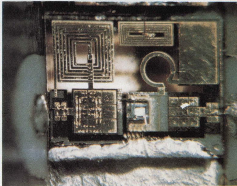
Big shrink. Breadboard version of hybrid 2-GHz amplifier with lumped elements is almost 1/40th the size of an equivalent unit made of conventional \frac{3}{4} x1" microstrip.
