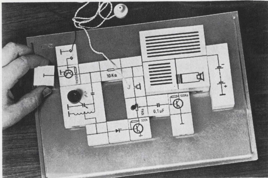
Broadcast band. Among the projects that amateur experimenters can build with their Lectron kit blocks is this three-transistor radio with loudspeaker.
