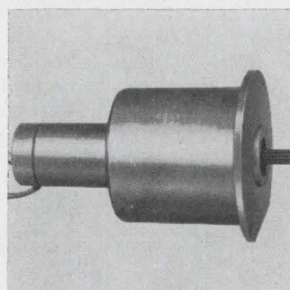
Servomotor tachometer size 23 is for use in power servo actuators. The 8-pole motor has a stall torque of 16 oz. in., and a free speed of 5,000 rpm. The tachometer produces an output of 2 v \pm 1\% per 1,000 rpm, has a phase shift of 0^{\circ} \pm 1^{\circ} , and linearity of \pm 7\% , and requires 5w of power. Operating temperature is -55^{\circ} to +132^{\circ} C. Weston-Transicoil, Worcester, Pa. [347]
