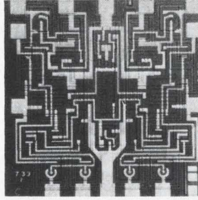
Dual operational amplifier #A739 is a linear IC that achieves high packing density with a 14-lead dual in-line package, which contains 2 identical op amps on a single silicon chip. Stable gain is maintained over a supply voltage range of ±4 to ±15 v. Power supply rejection is 50 μv/v. Slew rate is 1 v/μsec. Fairchild Semiconductor, 313 Fairchild Dr., Mtn. View, Calif. [438]
