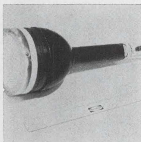
Cathode-ray projection tube CK1459P- is for video presentations on screens up to 10 to 20 sq ft in size. Television, radar, or computer-generated electronic information can be displayed. It uses a special face panel with high thermal conductivity to obtain a marked increase in light output, resolution, and tube life. Raytheon Co., 465 Centre St., Quincy, Mass. 02169. [346]
