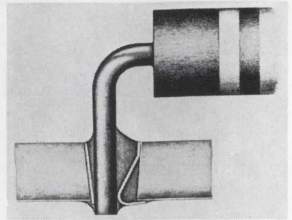
Gripping. Component lead is firmly held by springlike tension on fillet.
