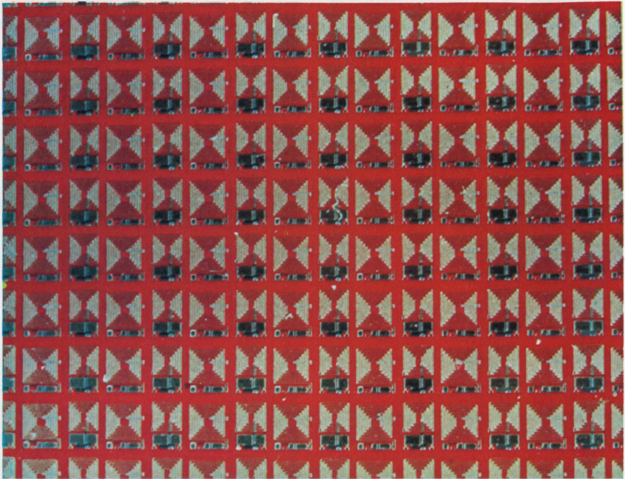
Lumped and batched. Passive elements of a 1-watt, 400-Mhz amplifier can be batch processed. Some 160 circuits fit on a 1-inch-square substrate.
