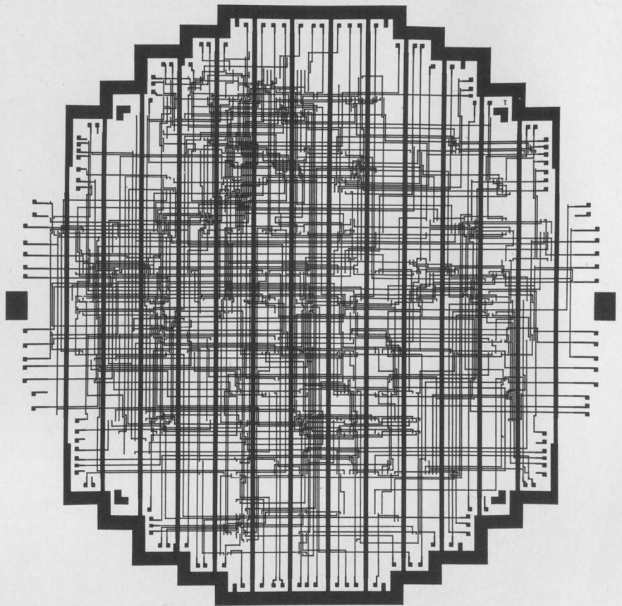
All lined up. A composite of the two masks for a typical circuit in the computer. CRT traces the hundreds of paths in just 132 seconds.
