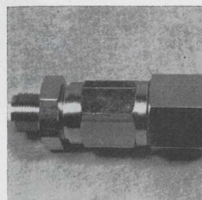
High voltage connectors series KV are less than 1 inch in diameter and will withstand 30 kv in a mated or unmated condition. They are available for various cable sizes—both flexible and semi-rigid—up through 3 inches. The connectors offer a pulse reflection coefficient of less than 1% maximum. General RF Fittings, Connector Division, Cove Road, Port Salerno, Fla. 33492. [344]
