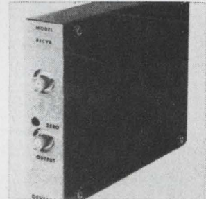
Light-coupled data amplifiers models 6110 and 6120 employ fiber optics to transmit data via a light pipe. Major system features include: common mode rejection greater than 100 db at 50 Mhz; frequency response d-c to 50 Mhz direct, or 20 to 80 khz f-m; 500,000 v common mode voltage isolation available. Develco Inc., 2433 Leghorn St., Mountain View, Calif. [424]
