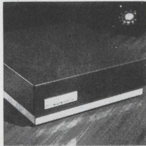
Data set called Modem 2200/24 transmits 2400 bps data over either dial-up or dedicated leased telephone lines. It is compatible with most existing four-phase units such as the Western Electric 201B. It includes circuit techniques formerly exclusive to the company's eight-phase data sets. Price is $2,350. International Communications Corp., 7620 N.W. 36th Ave., Miami, Fla. [422]
