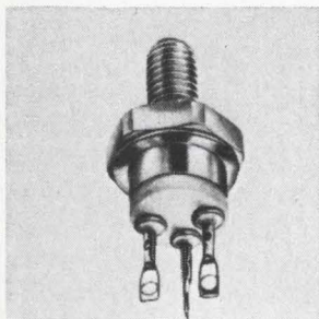
Isolated-collector, stud-mounted silicon transistors 2N5346-9 are medium-power npn devices with minimum f T 's of 30 Mhz. V CEO ranges from 80 to 100 v. Minimum beta at a collector current of 2 amps ranges from 30 to 60. Units are housed in a TO-59 package. Prices are between $24 and $34.95 in quantities of 100. Motorola Semiconductor Products Inc., Box 20924, Phoenix. [440]
