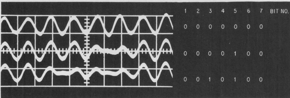
Data pulses. In one test, pulses generated by passing sonic wave represent binary 0's; where a 1 no pulse. Scales are 0.5 mv and 0.2 \mu sec per division.
