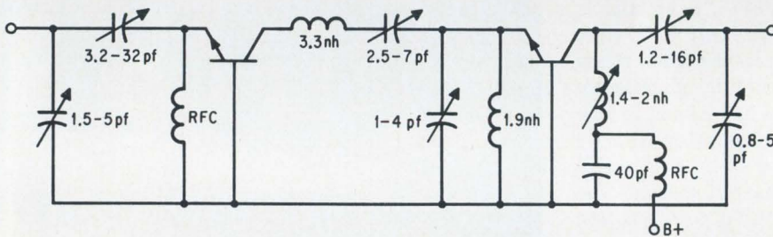
Lumped and batched. Passive elements of a 1-watt, 400-Mhz amplifier can be batch processed. Some 160 circuits fit on a 1-inch-square substrate.
