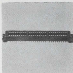
P-c connector series 600-121-27 is a 27-dual contact unit (54 terminals) with 0.100 in. center-to-center contact spacing. A choice of dip solder or solder lug terminations is available in gold plated beryllium copper. Glass reinforced diallyl phthalate molding type GDI-30 per MIL-P-19833 has 3 integral polarizing barriers. Continental Connector Corp., Woodside, N.Y. [343]
