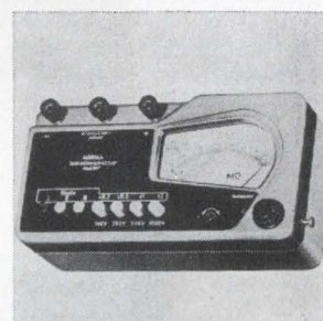
Portable megohmmeter type 667 is battery operated and suited for making accurate insulation tests of motors, wiring, appliances and other electrical equipment. Four test voltages are available: 100, 250, 500 and 1,000 v d-c with a resistance range from 0 to 10,000 megohms at 500 v d-c. Price is $175. Freed Transformer Co., 1718 Weirfield St., Brooklyn, N.Y. 11227. [364]
