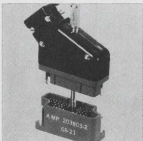
High density rectangular connector series HDR in 54-contact size features crimp-and-insert contacts on a 100-in. square grid pattern. Size 20 contacts are rated at 7.5 amps and come in two wire range sizes, 20-24 and 24-30 Awg. Contact plating is gold over nickel, selective gold, or tin. Housings are black phenolic or blue diallyl phthalate. AMP Inc., Harrisburg, Pa. [345]
