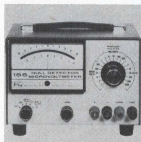
Combination null detector/micro-voltmeter model 155 offers 1 \mu v full scale sensitivity to 1000 v range. It features less than 150 nv noise, greater than 140 db common mode rejection ratio, and greater than 100 db normal mode rejection ratio, and greater than 10^{12} ohms isolation from ground. Price (1-4) is $325 each. Keithley Instruments Inc., 28775 Aurora Rd., Cleveland. [367]
