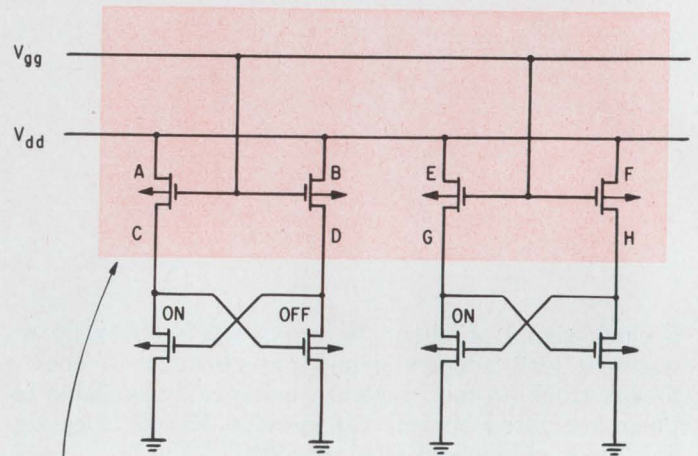
TINTED AREA SHOWN IN MASK LAYOUT
