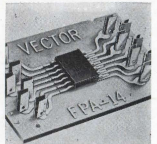
Flatpack adapters are for mounting 14-lead IC's on circuit boards. The adapter is a 1/16-in. epoxy paper wafer with a 2-oz. copper etched pattern which matches the 0.05-in. spaced lead pattern on flatpacks. Price for small quantities is 53 cents per wafer in packages of four. Units are available from the factory. Vector Electronic Co., 12460 Gladstone Ave., Sylmar, Calif. [348]
