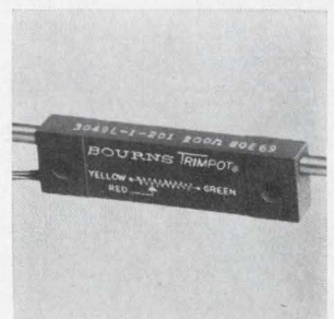
Cermet element, position pot 3049 has a \frac{1}{2} -in. nominal stroke with mechanical life of 20,000 cycles and \pm 2\% standard linearity. It is expected to find wide acceptance in industrial controls and lab-type applications. Resistance range is 100 ohms to 1 megohm. Power rating is 1 w at 70^\circ C. Price (500 lots) is $4.65 each. Bourns Inc., 1200 Columbia Ave., Riverside, Calif. [428]
