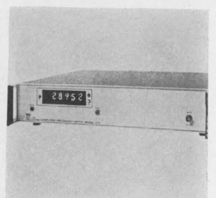
Computing frequency meter model 270 has no knobs and no adjustments, only a power switch and a reset button. To measure any frequency between 1 hz and 1 Mhz, one needs only to turn on the power, connect the input signal, read the frequency to 5 significant digits, and measurement takes only 1 second. Time Systems Corp., 265 Whisman Rd., Mountain View, Calif. [368]
