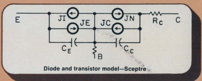
Hybrid model for transistor
