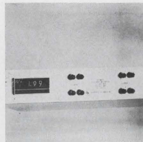
Digiwatt Halltiplier wattmeter provides not only digital panel meter readout but two output signals as well. The output signals are 0 to 100 mv d-c analog signal and a BCD 1-2-4-8 output. Units are single-range, two-element, three-phase devices which provide highly accurate measurements of electrical power. Scientific Columbus, 1035 W. 3rd Ave., Columbus, Ohio. [363]
