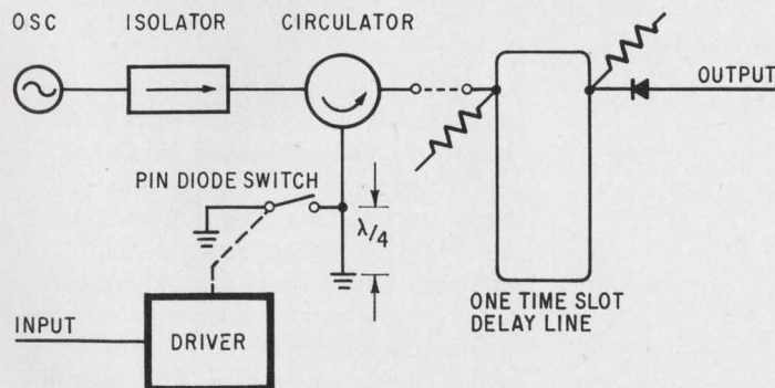
Proper path. Path-length modulation of an Implatt diode uses a p-i-n diode as a switch to change the phase of the millimeter wave. The input to the diode is the baseband signal; the output of the time slot delay line is a baseband-modulated signal.
