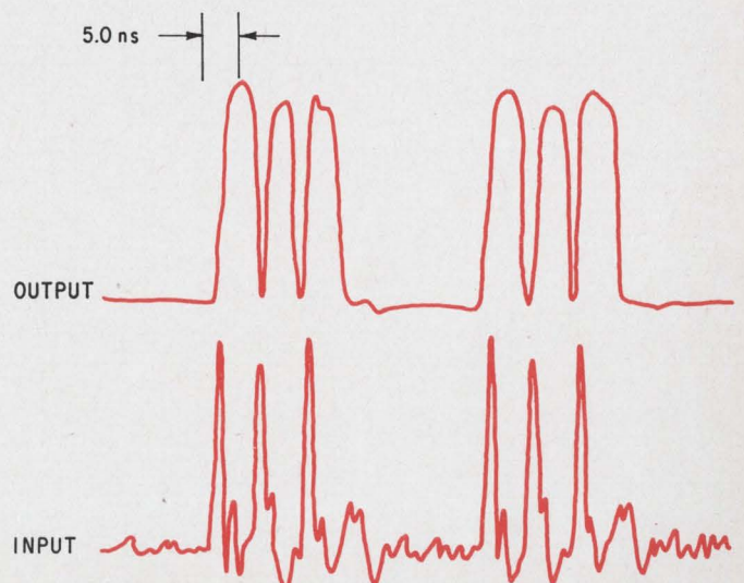
Proper path. Path-length modulation of an Implatt diode uses a p-i-n diode as a switch to change the phase of the millimeter wave. The input to the diode is the baseband signal; the output of the time slot delay line is a baseband-modulated signal.
