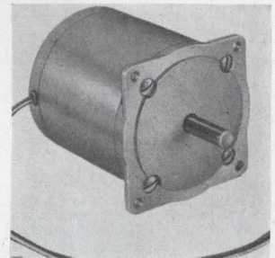
Slo-Syn synchronous/stepping motor type LS50 has a low shaft speed of 28.8 rpm at 60 hertz without step-down gearing. Used as an a-c motor it will start, stop, and reverse almost instantly. The motor will stop within 25 msec without external braking. It is rated for 120 v 0.2 amp. It features 40 oz-in. torque. Superior Electric Co., 382 Middle St., Bristol, Conn. 06010 [424]
