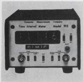
Time interval meter model 915 has a 1-Mhz temperature compensated crystal oscillator. It triggers on positive or negative going pulses, and can be operated in either a 1\mu\text{sec} or 1 msec mode, with a range from 0 to 99,999. Measurements start on A-input and stop on B-input. Price is $555. Computer Measurements Division, Newell Industries, Bradley Ave., San Fernando, Calif. [361]
