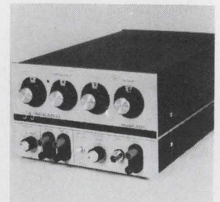
Digital oscillator series 2000, because of its versatility in control and setting, is suitable for in excess of 90% of all sine wave signal generation requirements in the range from 10 hz to 12 Mhz. Frequency selection is accomplished by digital front panel switches. Unit comes in a half rack package. J&J Instruments, 8141 Engineer Rd., San Diego, Calif. 92111. [364]
