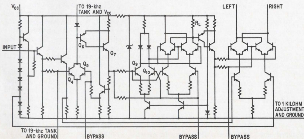
On a chip. Part of new line of consumer IC's from Mitsubishi, stereo multiplex IC has about 60 transistors. Only part of the total circuit is shown here. Main design feature is elimination of a 38-khz auxiliary tuned circuit.
