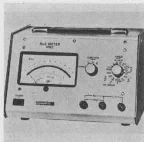
Direct reading RLC meter MM2 performs resistance measurements in 12 linear ranges from a virtual short circuit at 0.1 ohm to 1 megohm. Inductances are measured in 16 linear ranges from 3\mu\text{h} to 100 henrys full scale. Capacitance measurements also cover a dynamic span, in 16 ranges, from 3 pf to 100\mu\text{f} with linear readings throughout. The London Co., Sharon Dr., Cleveland [366]
