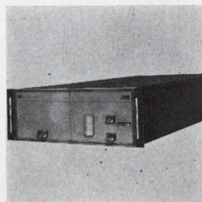
Digital printer AN72 is designed to interface with a wide variety of equipment. For example, it can be fed with 4-line, 5-line, or 6-line BCD data. If a 4-line input is used, the printer can print all the decimal digits plus 6 additional signs and symbols. For standardization, input follows an ASCII format. Datadyne Corp., Valley Forge Center, King of Prussia, Pa. 19406 [405]
