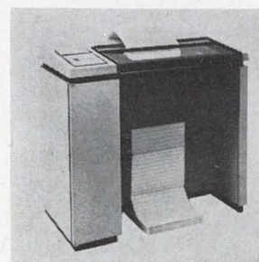
Line printer model 2410 is a 132-column unit designed for use with small/medium size computers and data communications terminals. The company's Mark IV print hammer provides printing speeds of 245 to 1110 lines a minute for all 64 characters. A drum speed of 1,760 rpm allows for a time sharing of electronics. Data Products Corp., 6219 DeSoto Ave., Woodland Hills, Calif. [407]
