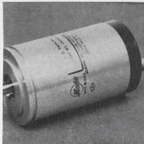
Size 18 d-c tachometer CVO 9612 001, for industrial applications, features a high output of 100 v per 1,000 rpm and exhibits low-ripple voltage. Used for feedback-drive or velocity servo-drive functions, it serves as an integral part of a contour-control system. Ambient temperature range is -54^\circ to +100^\circ C. Singer-General Precision Inc., Kearfott Division, Little Falls, N.J. [423]
