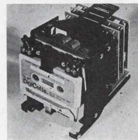
Tape transport called DigiDeck has two independent bit serial data recording channels which may be operated simultaneously or independently in various modes. It brings the speed and convenience of magnetic tape to small data systems requiring an accurate, low-cost method of storing and retrieving digital data. International Computer Products Inc., Box 34484, Dallas [406]
