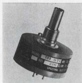
Single-turn, cermet precision pot model 139 features a high-power rating suited for industrial use in controls and instrumentation. It offers a resistance range of 500 ohms to 1 megohm, essentially infinite resolution, and a standard independent linearity of \pm 0.5\% . Power rating is 5 watts at 40^\circ C. Spectrol Electronics Corp., 17070 E. Gale Ave., City of Industry, Calif. [426]
