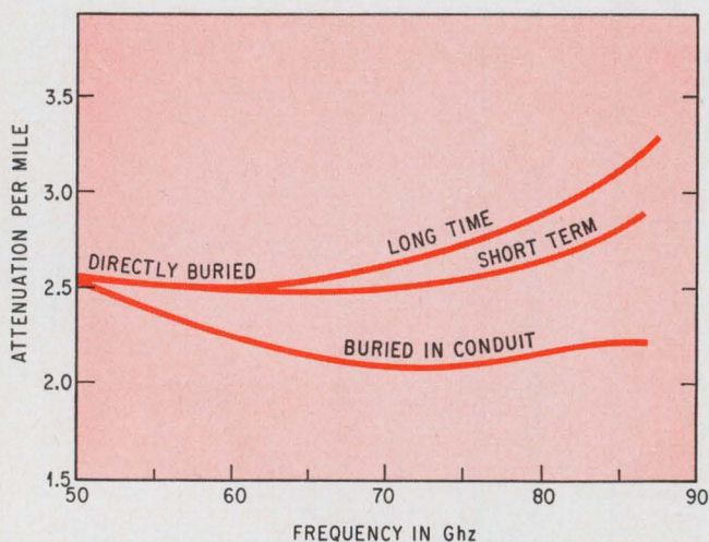
Buried alive. By burying the waveguide in a conduit, attenuation over the long term is reduced by 0.6 decibels and 0.3 db over the short term.
