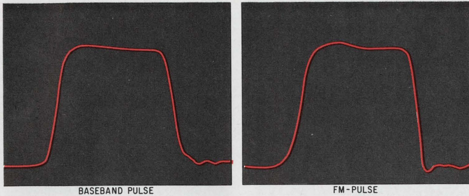
True Grit. Direct frequency modulation of the Impatt diode—variation of the oscillation frequency by varying the bias current—can be accomplished with almost no distortion of the original modulating baseband pulses. An input baseband pulse, left, before modulation, a detected f-m pulse, right, after modulation, show almost no increase in rise time or distortion.
