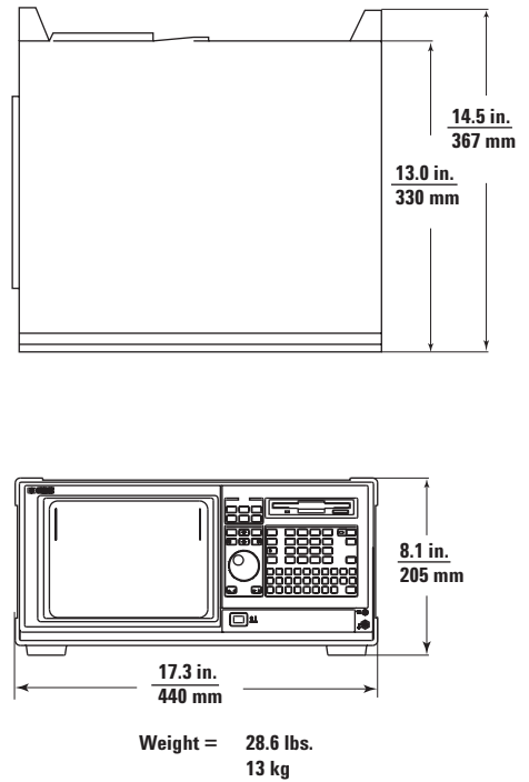
Figure 2. Logic Analyzer Dimensions and Weight
